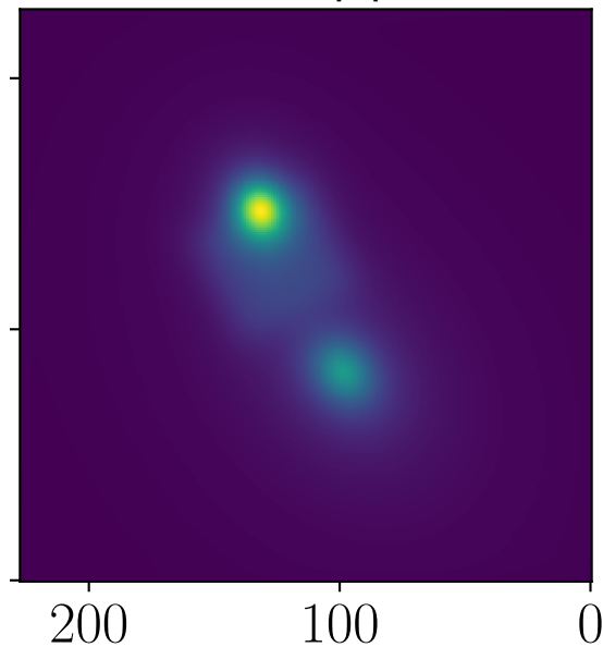
Model, Planck, npipe, 353 GHz
