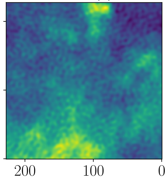
Residual, Planck, npipe, 353 GHz
