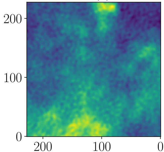
Data, Planck, npipe, 353 GHz
