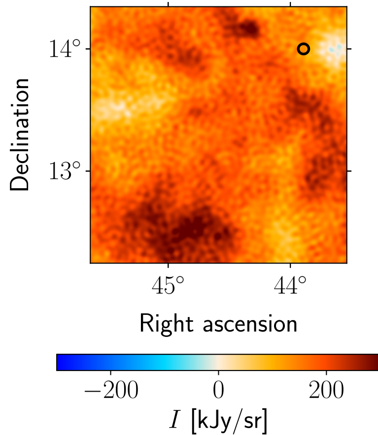
Residual: Planck 217 GHz
