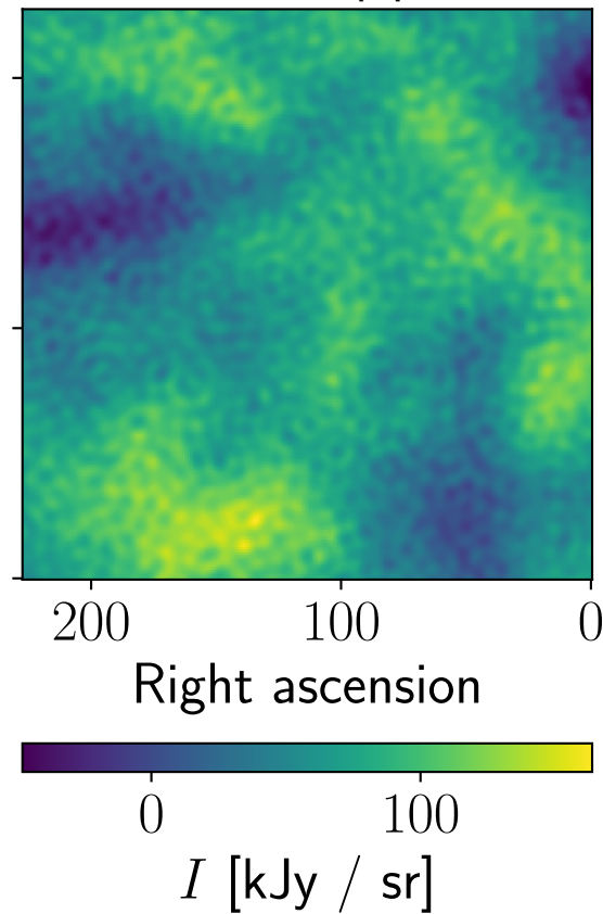
Residual, Planck, npipe, 143 GHz
