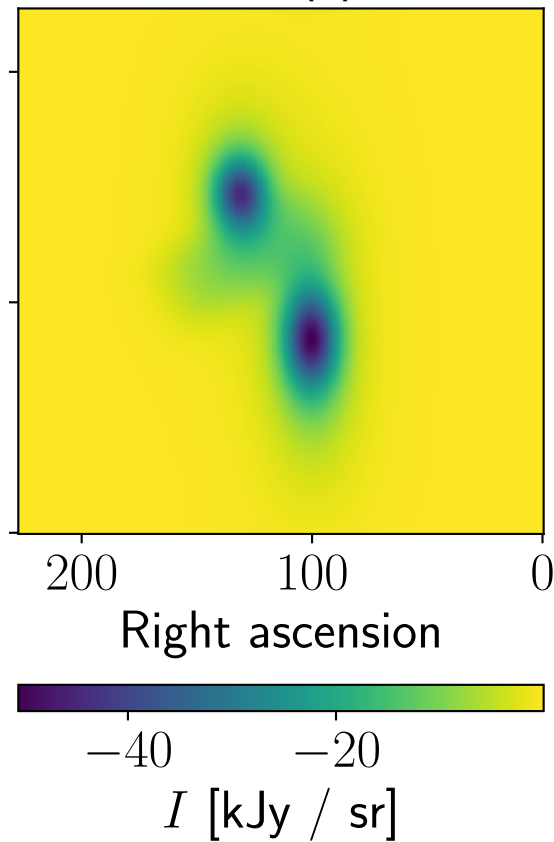
Model, Planck, npipe, 143 GHz
