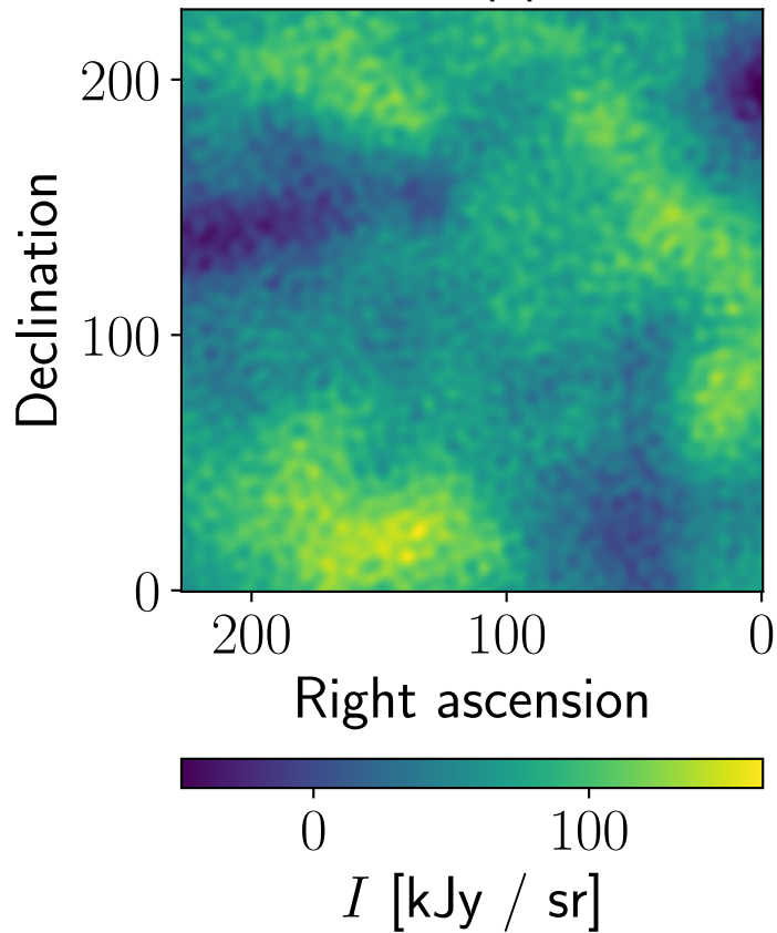
Data, Planck, npipe, 143 GHz
