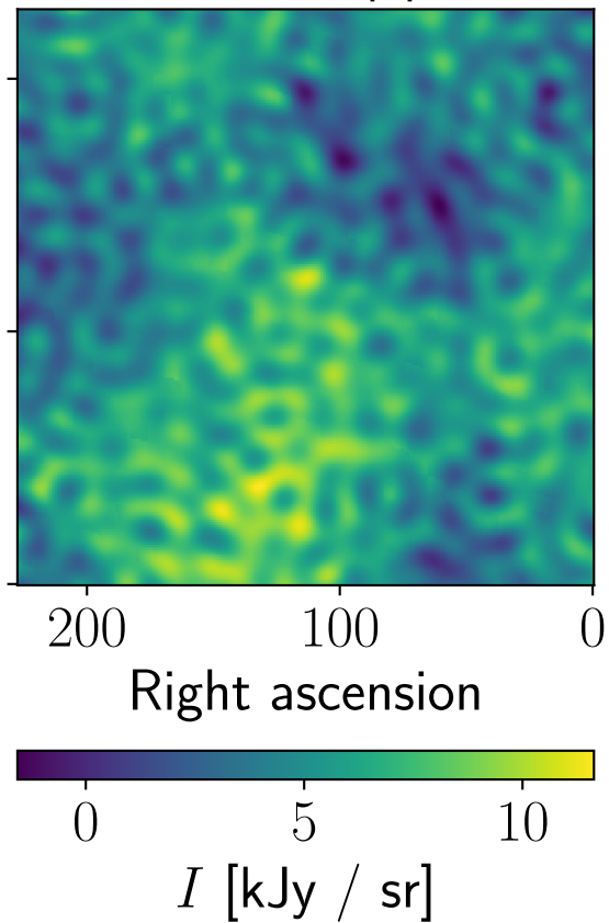
Residual, Planck, npipe, 30 GHz
