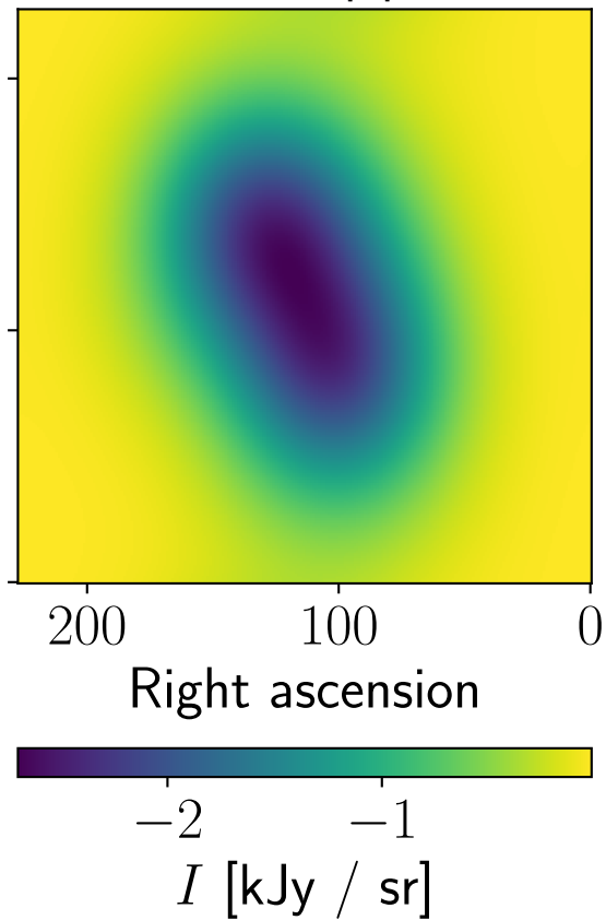
Model, Planck, npipe, 30 GHz
