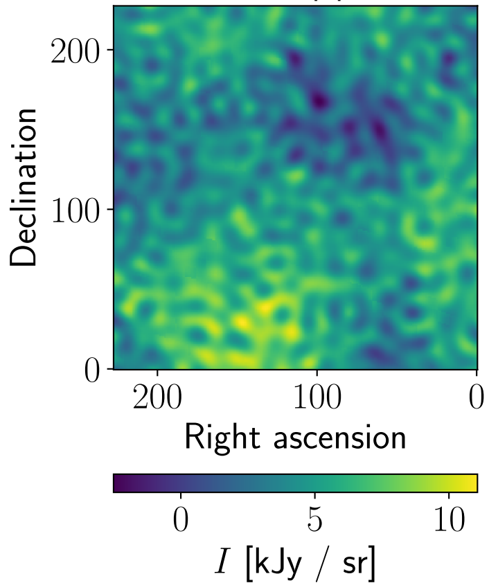
Data, Planck, npipe, 30 GHz
