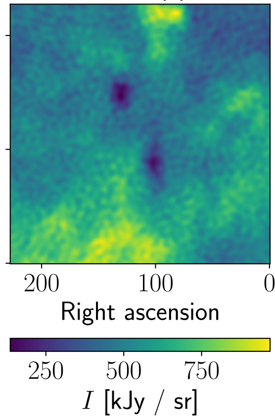
Residual, Planck, npipe, 353 GHz
