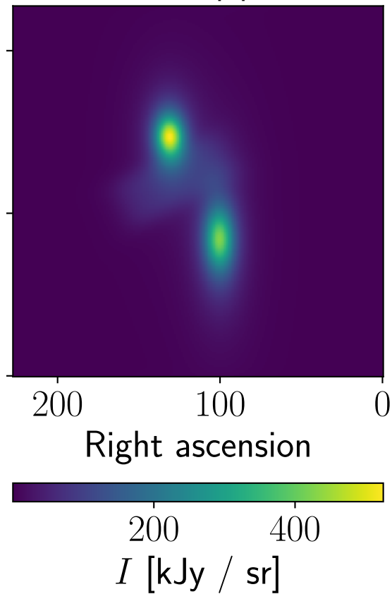
Model, Planck, npipe, 353 GHz
