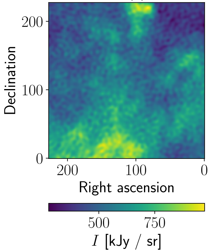
Data, Planck, npipe, 353 GHz
