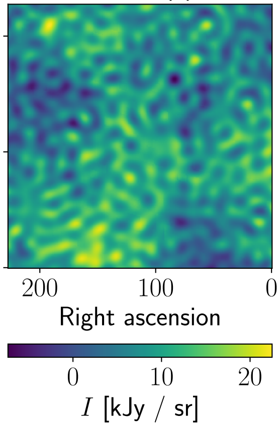
Residual, Planck, npipe, 44 GHz
