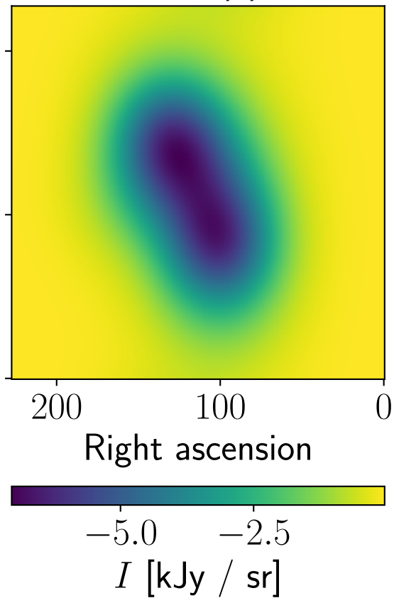
Model, Planck, npipe, 44 GHz
