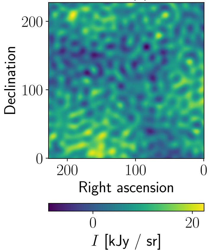
Data, Planck, npipe, 44 GHz
