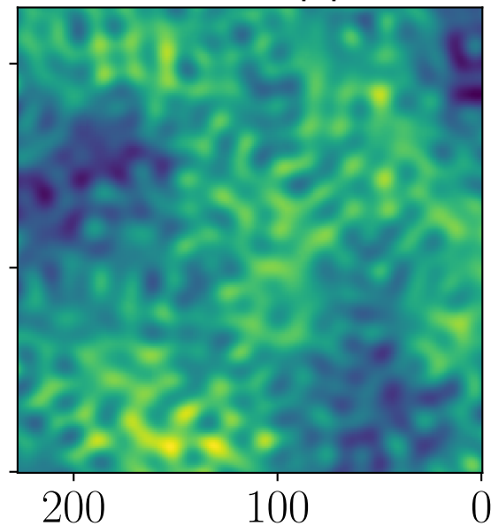
Residual, Planck, npipe, 70 GHz
