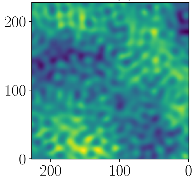
Data, Planck, npipe, 70 GHz
