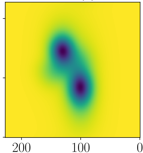
Model, Planck, npipe, 70 GHz
