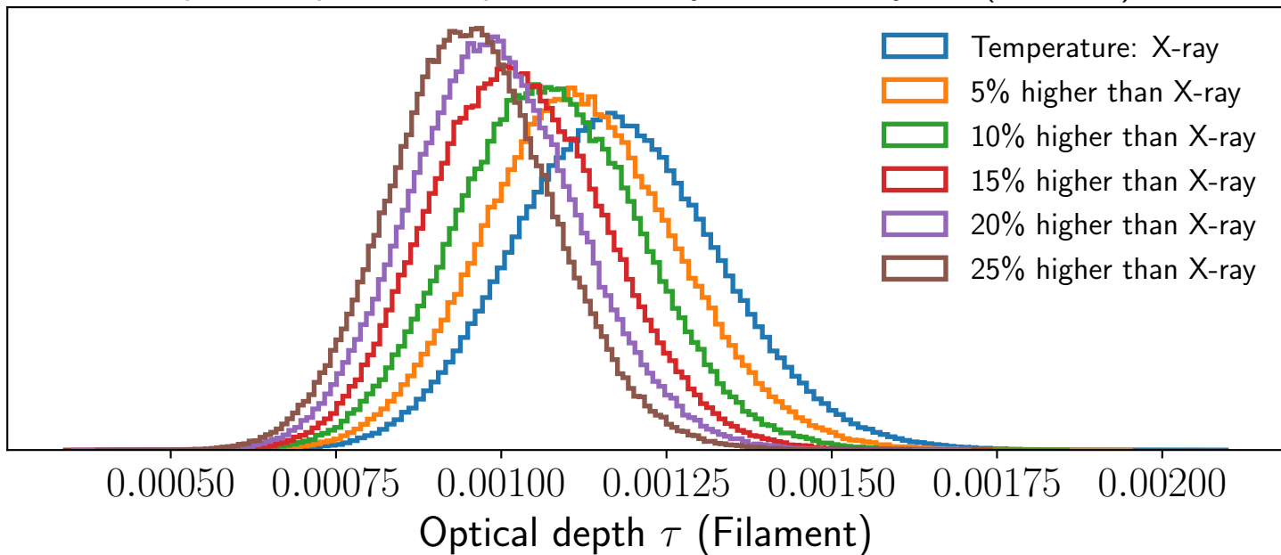
Optical depth vs temperature for system velocity fits (filament)
