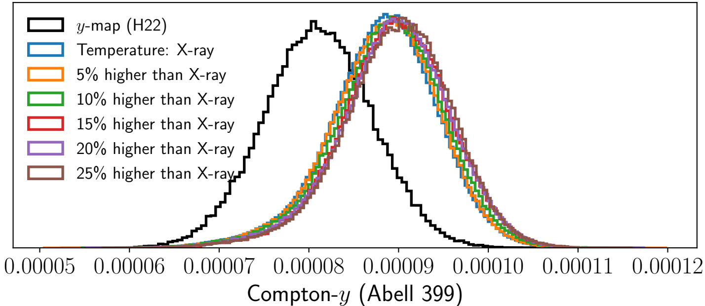
Compton- y vs temperature for system velocity fits (Abell 399)
