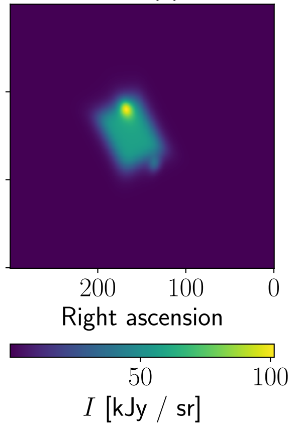
Model, Planck, npipe, 217 GHz
