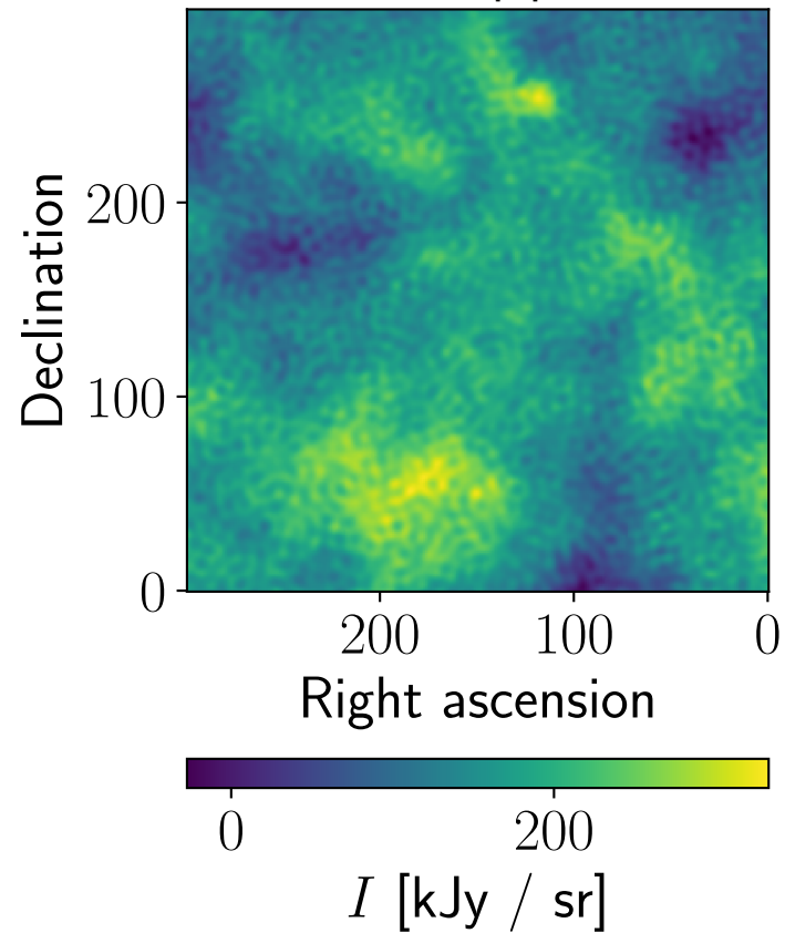
Data, Planck, npipe, 217 GHz
