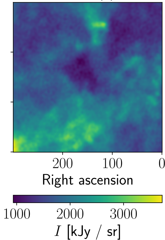
Residual, Planck, npipe, 545 GHz
