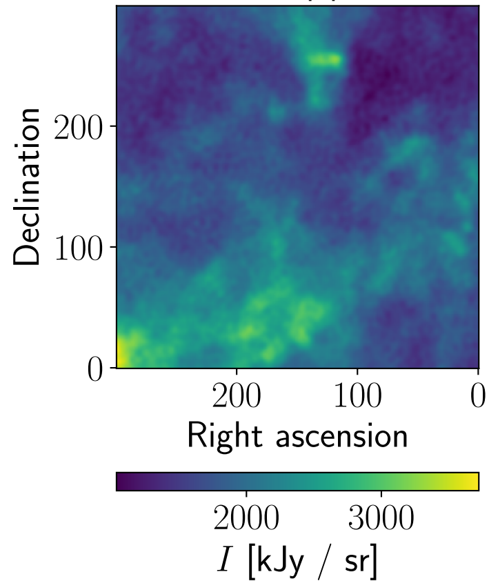
Data, Planck, npipe, 545 GHz
