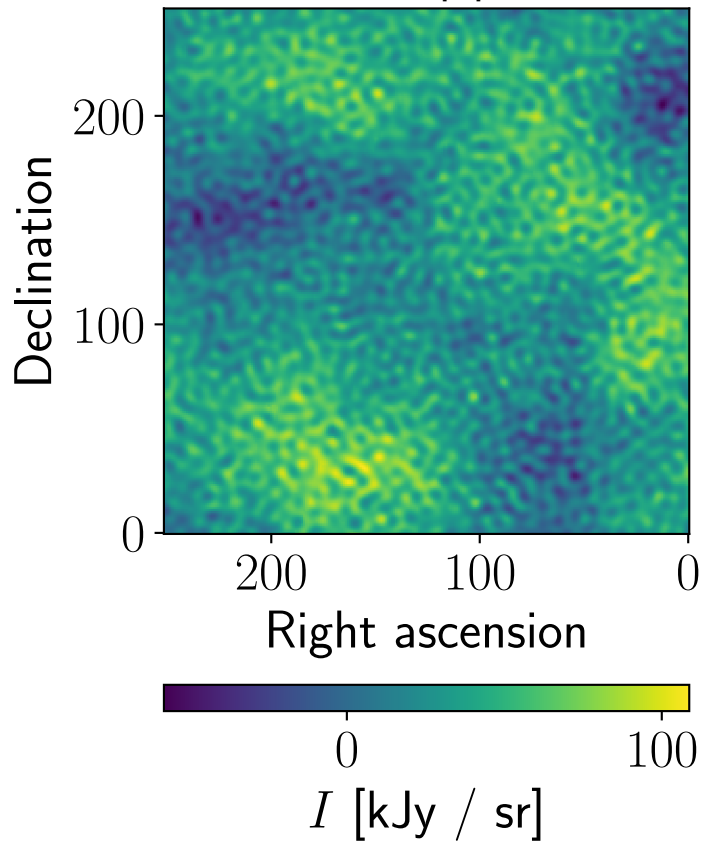
Data, Planck, npipe, 100 GHz
