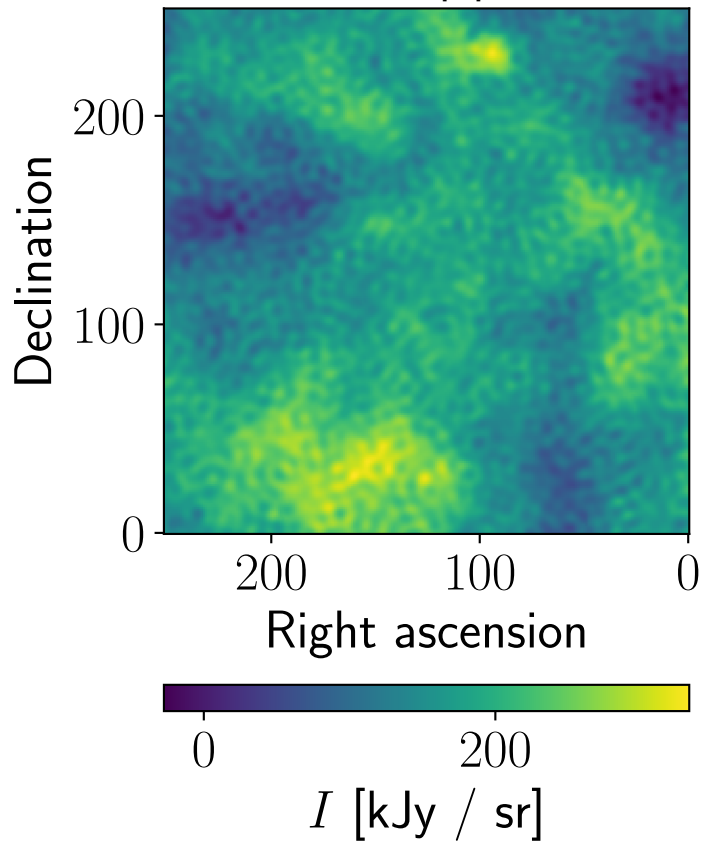
Data, Planck, npipe, 217 GHz
