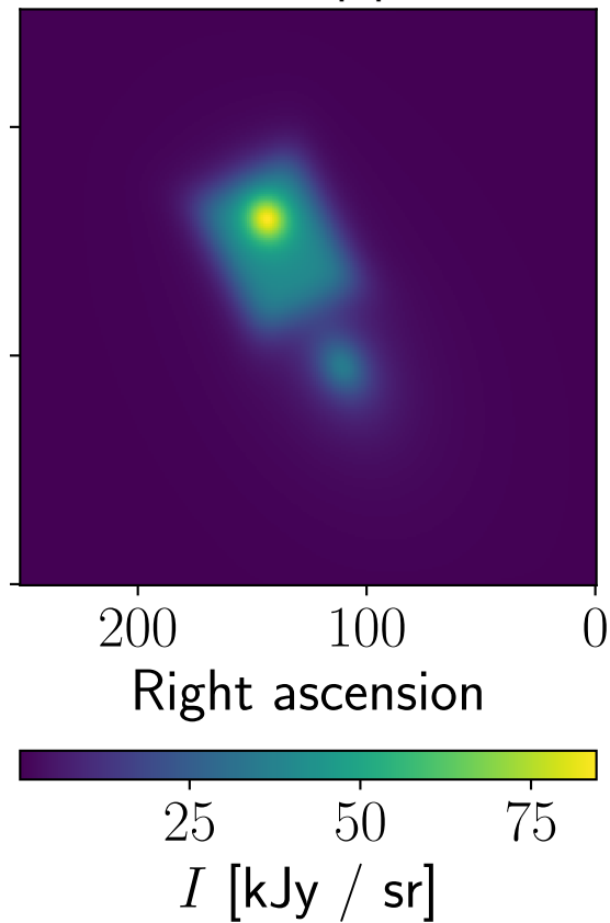
Model, Planck, npipe, 217 GHz
