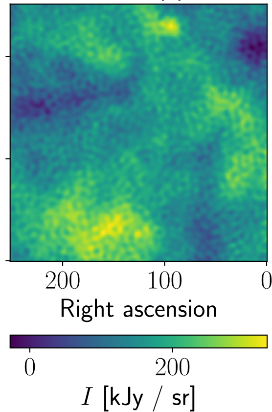
Residual, Planck, npipe, 217 GHz
