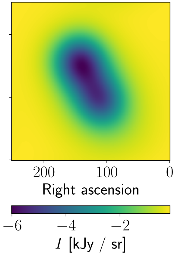
Model, Planck, npipe, 44 GHz
