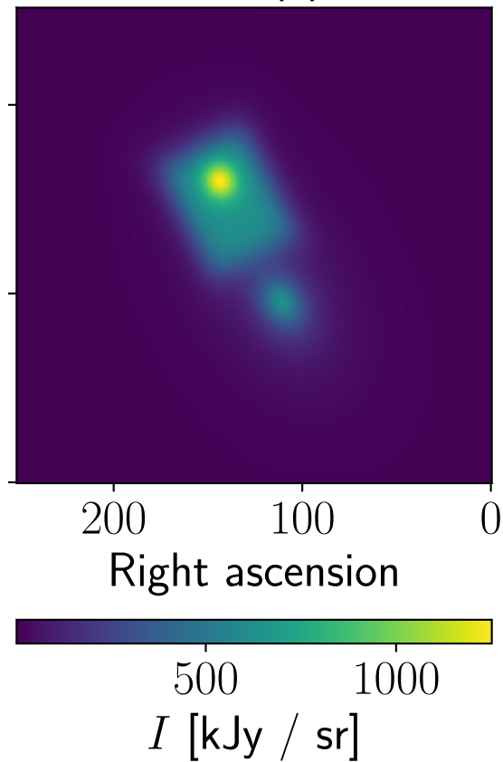
Model, Planck, npipe, 545 GHz
