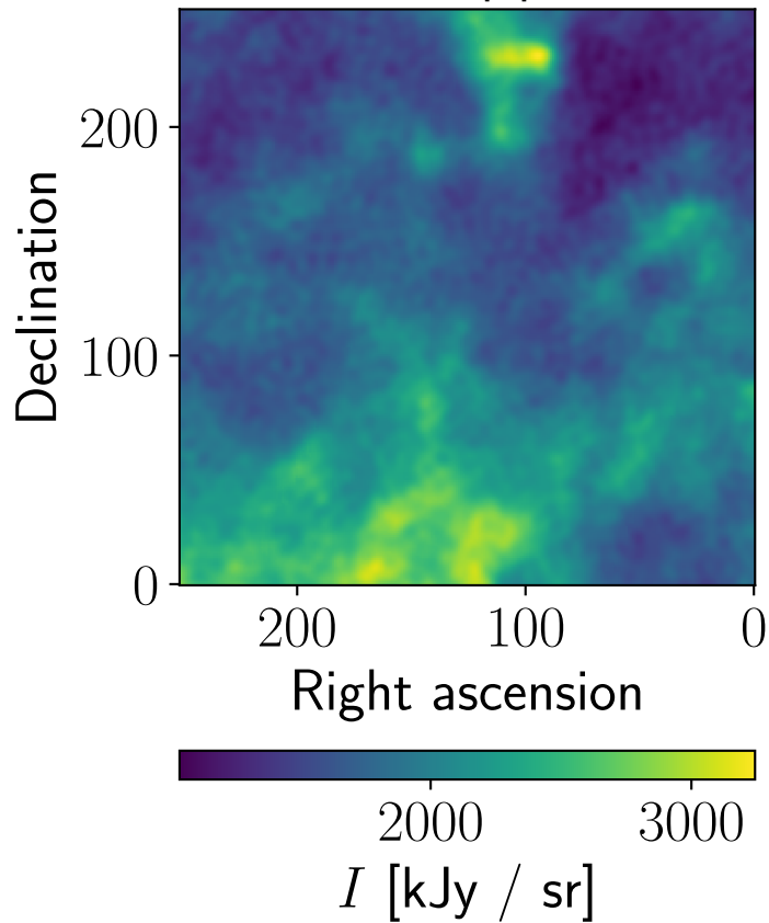
Data, Planck, npipe, 545 GHz
