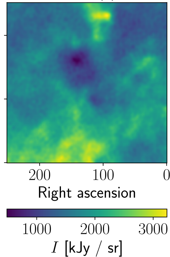
Residual, Planck, npipe, 545 GHz
