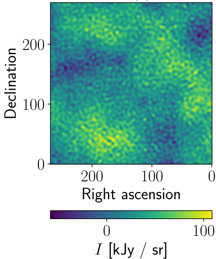
Data, Planck, npipe, 100 GHz
