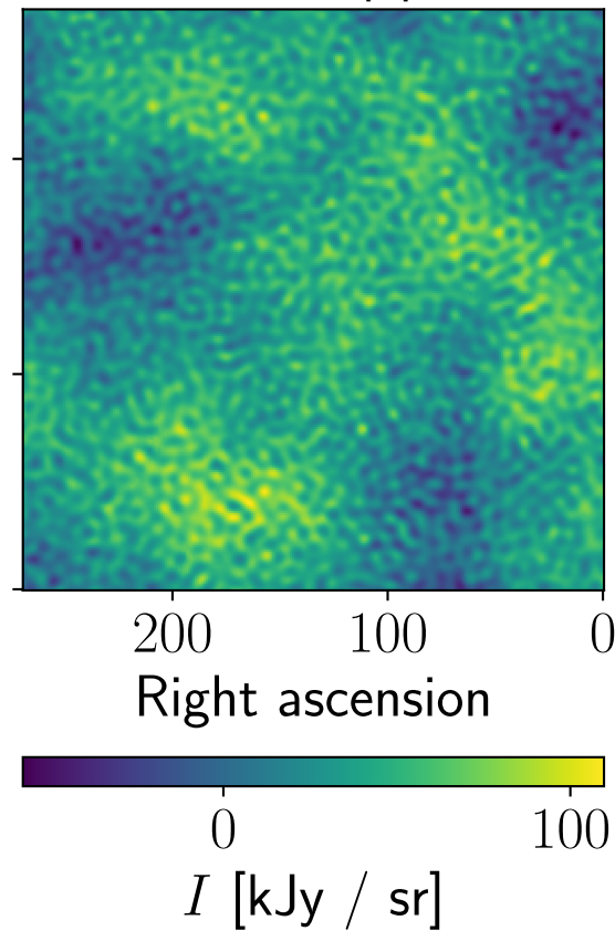
Residual, Planck, npipe, 100 GHz
