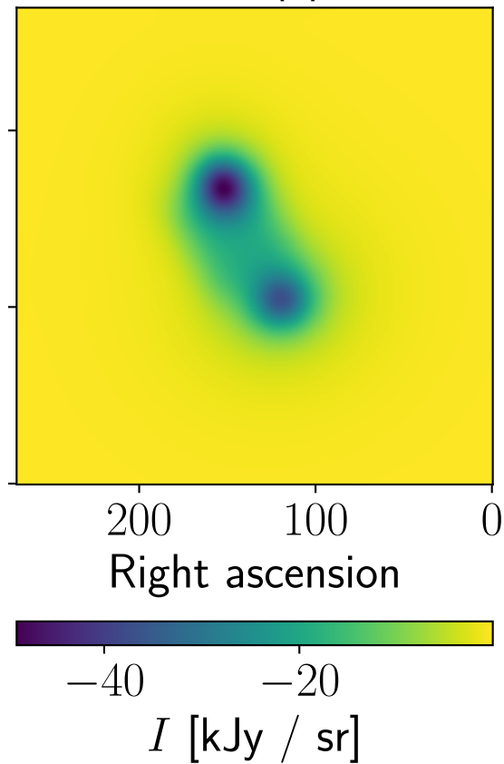
Model, Planck, npipe, 100 GHz
