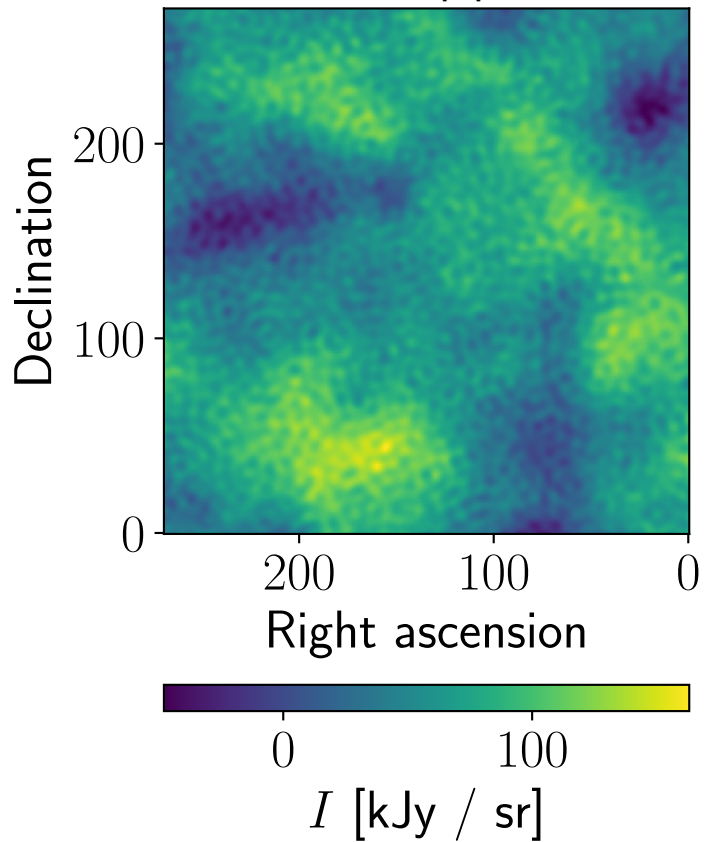
Data, Planck, npipe, 143 GHz
