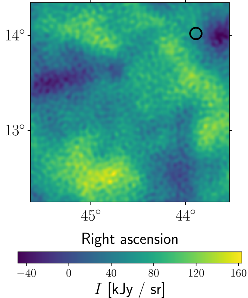
Data, Planck , 143 GHz
