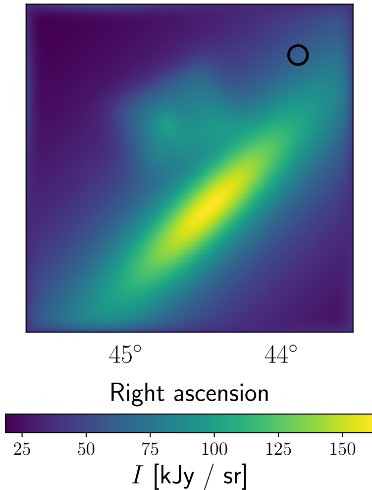
Model, Planck , 143 GHz
