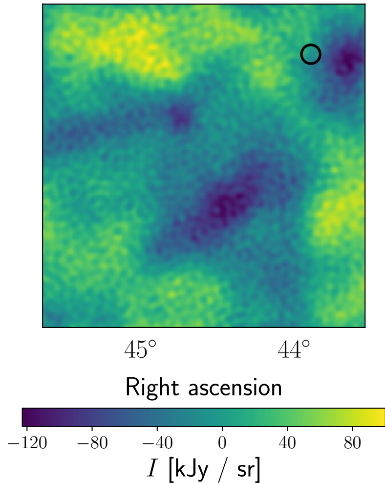
Residual, Planck , 143 GHz
