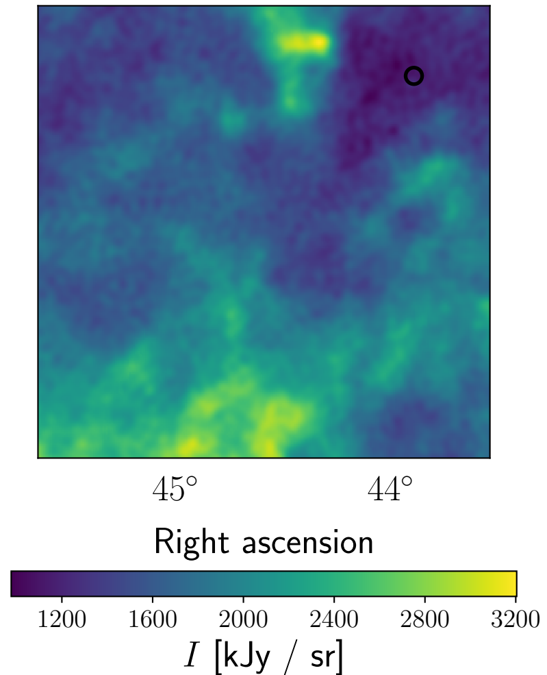
Residual, Planck , 545 GHz
