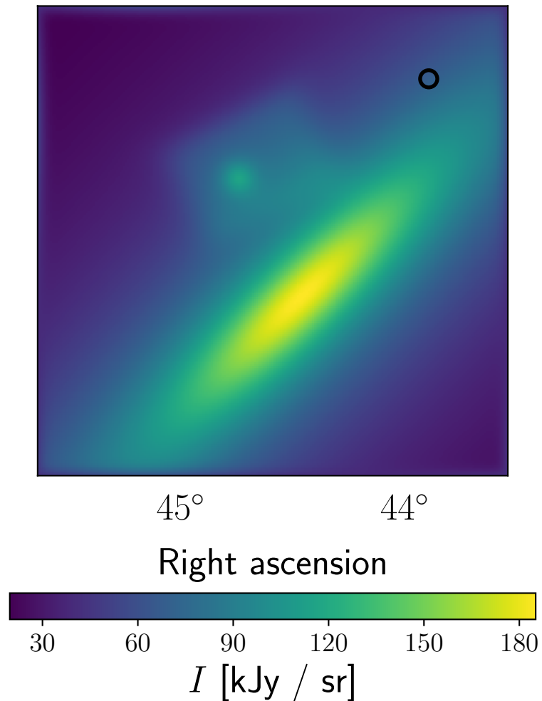
Model, Planck , 545 GHz
