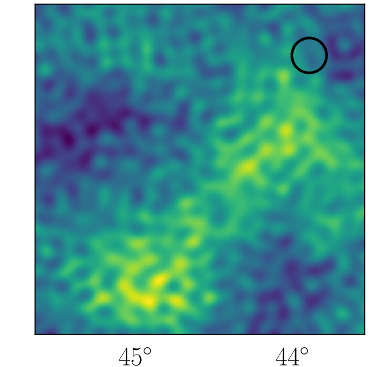
Residual, Planck , 70 GHz
