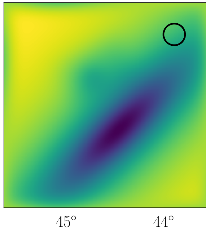
Model, Planck , 70 GHz
