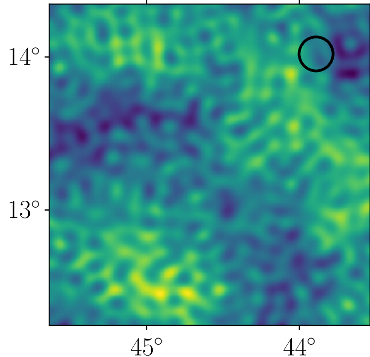
Data, Planck , 70 GHz
