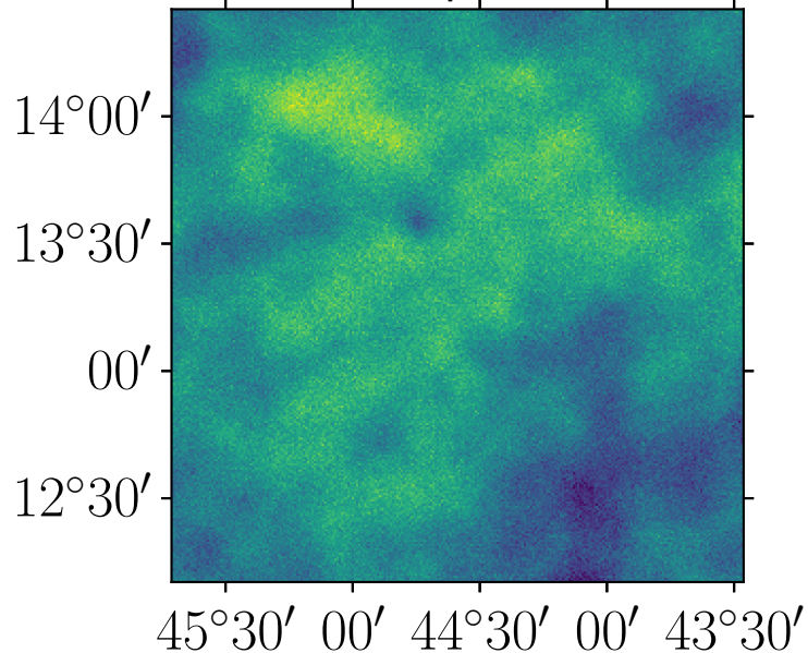
Data, ACT, pa5, 150 GHz
