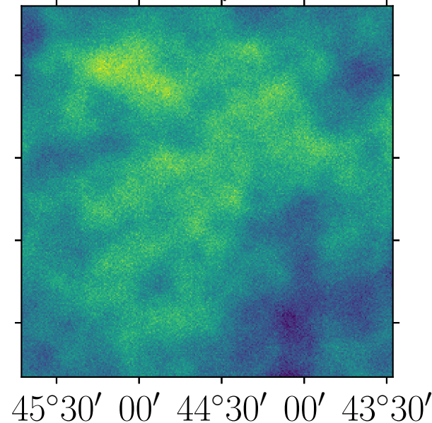
Residual, ACT, pa5, 150 GHz
