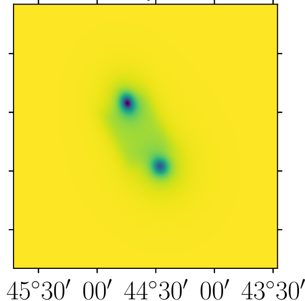
Model, ACT, pa5, 150 GHz
