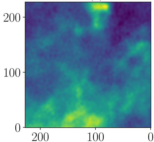
Data, Planck, npipe, 545 GHz
