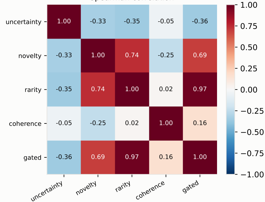
Spearman correlation
