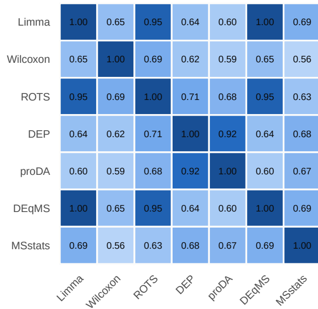
A. DEA methods are correlated, not independent
