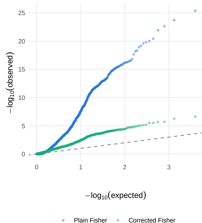
C. Plain Fisher inflates small p-values
