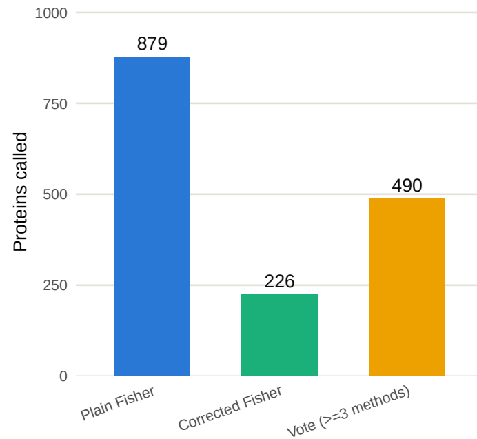
B. Plain Fisher over-calls DEPs
