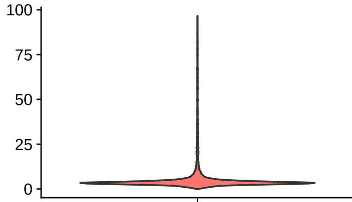
pct_mt
