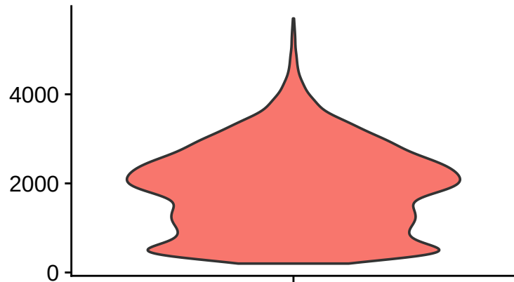
nFeature_RNA
