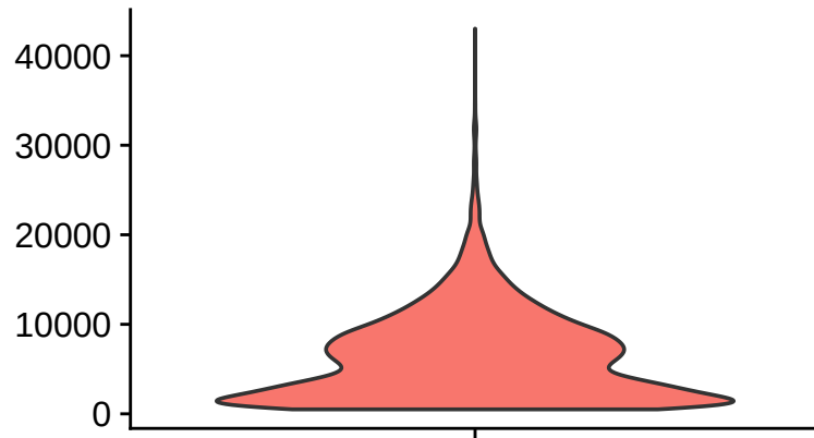
nCount_RNA
