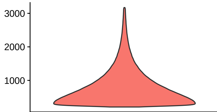
nCount_RNA
