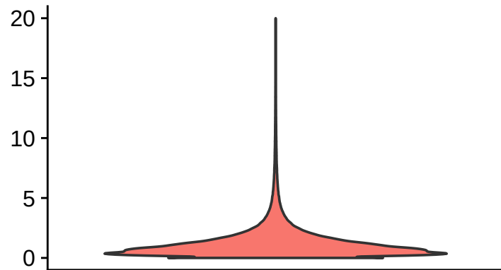
pct_mt
