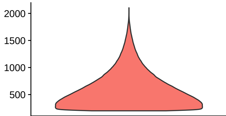
nFeature_RNA
