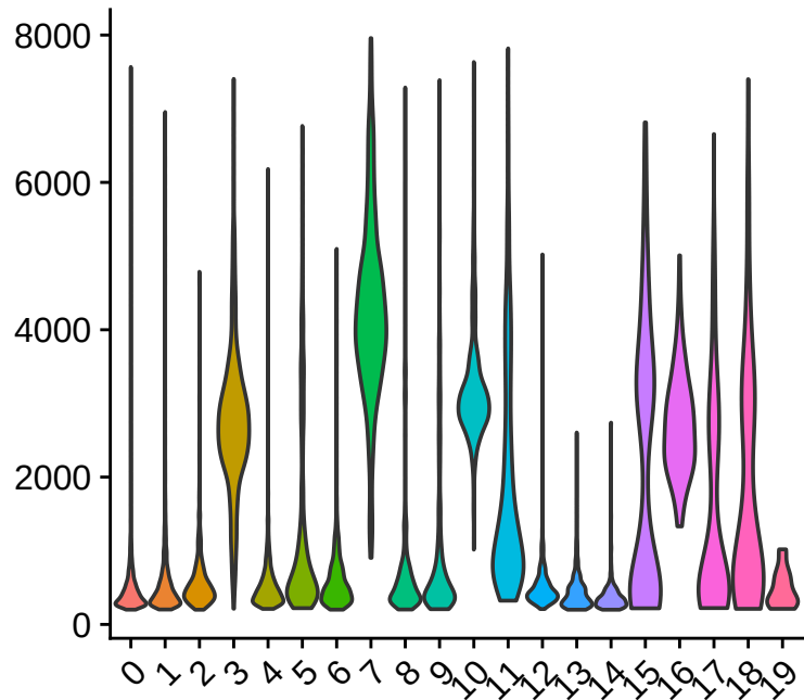
nFeature_RNA
