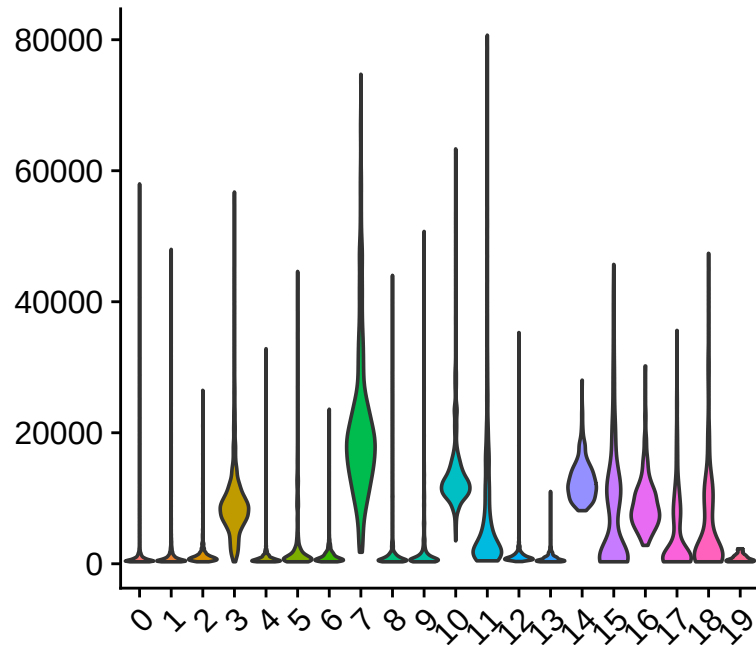
nCount_RNA
