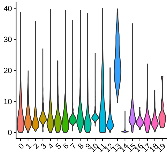
pct_mt
