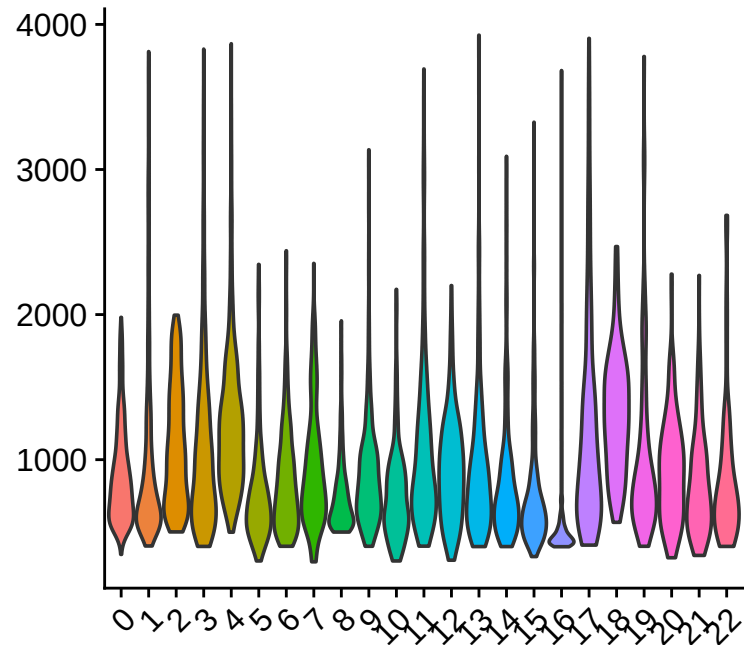
nFeature_RNA
