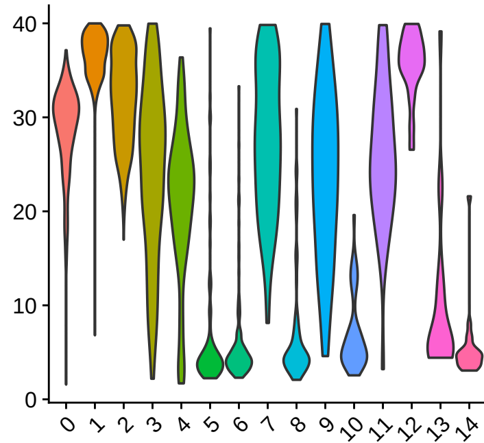
pct_mt
