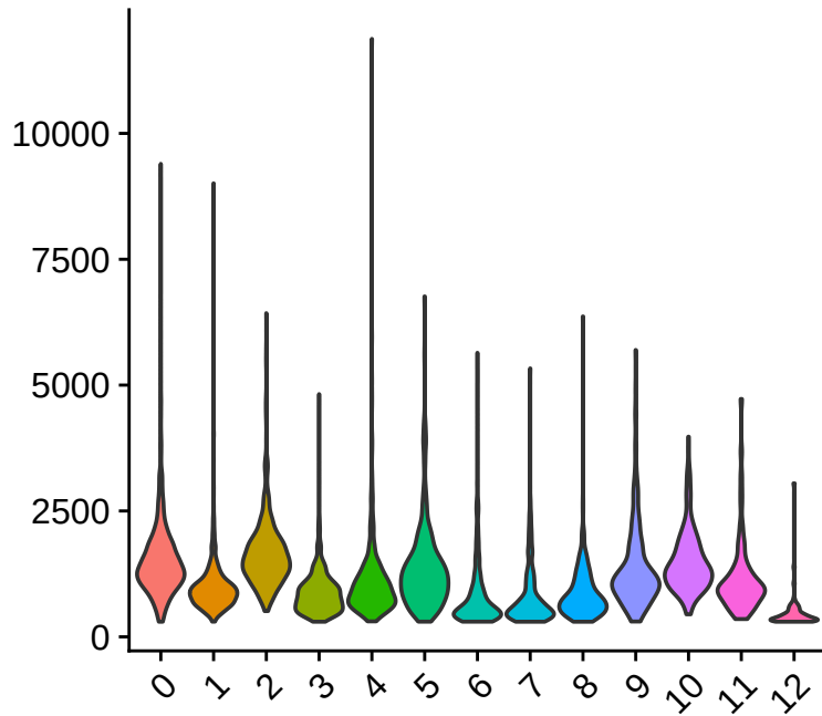
nCount_RNA
