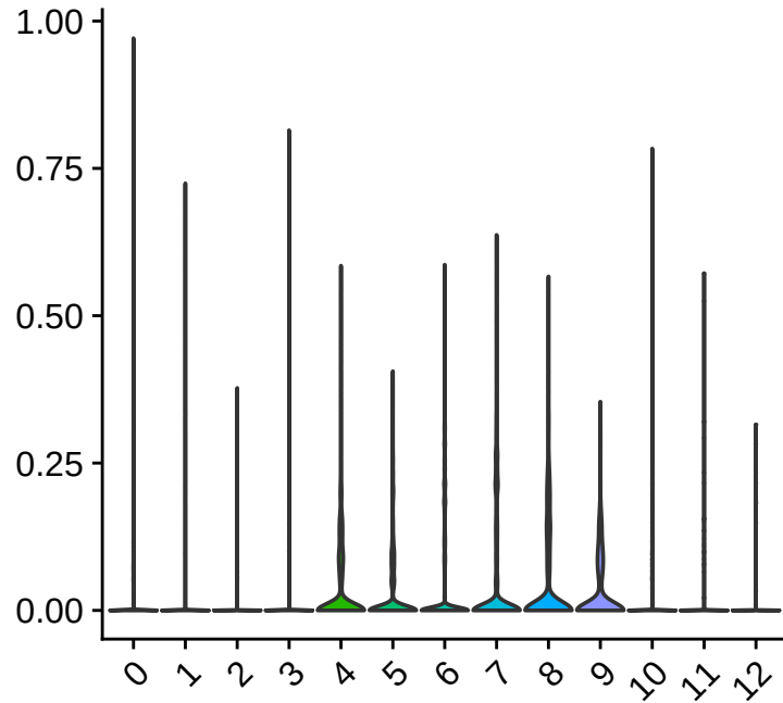
pct_mt
