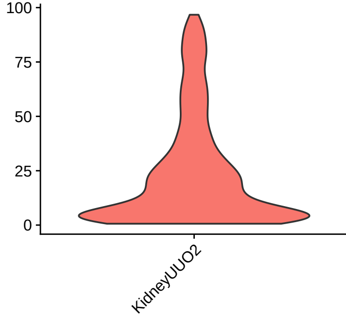
pct_mt
