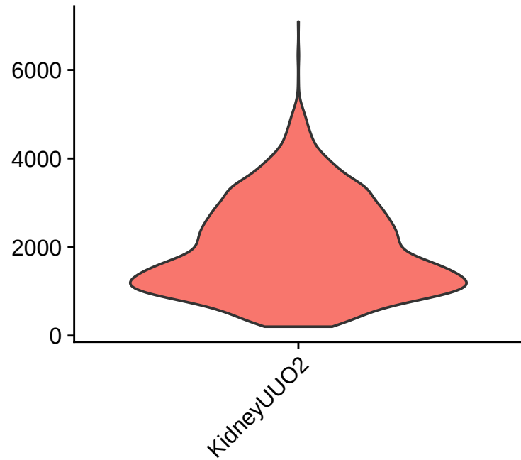
nFeature_RNA
