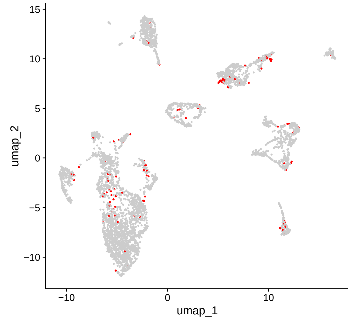
KidneyUUO3 – DoubletFinder
