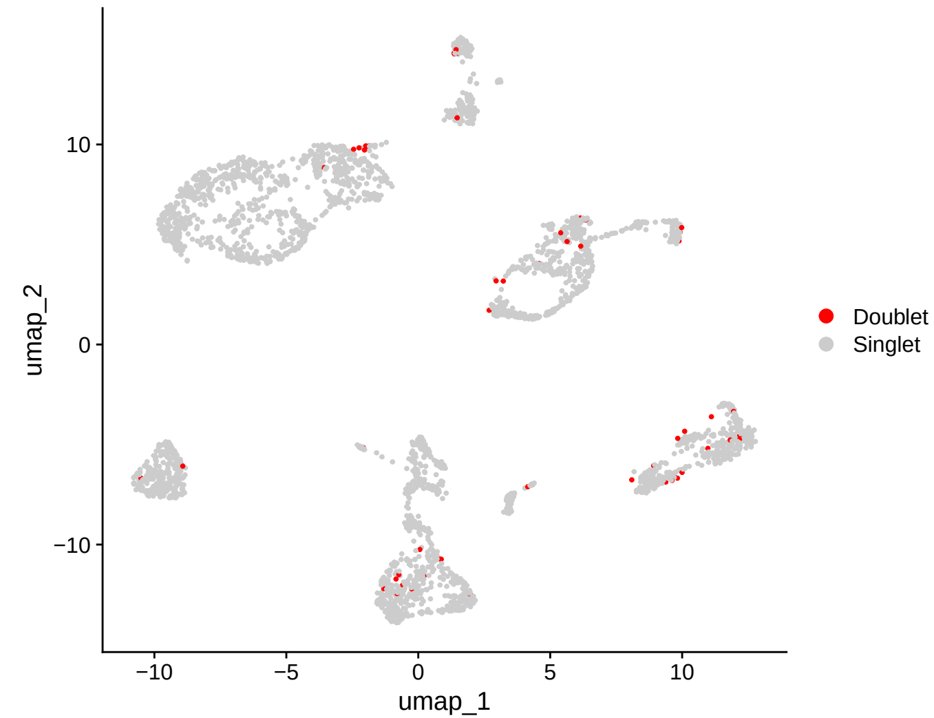
KidneyrUUO1 – DoubletFinder
