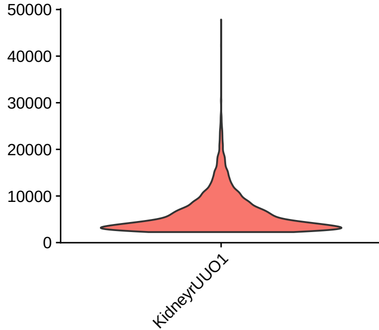
nCount_RNA
