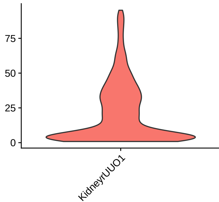
pct_mt
