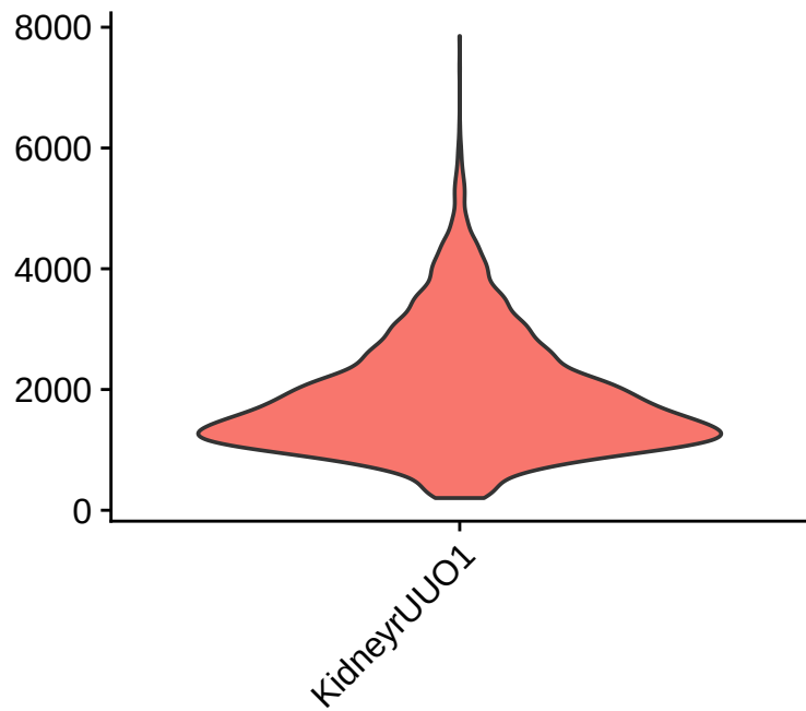
nFeature_RNA
