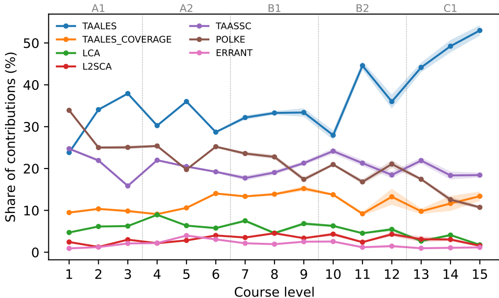
Feature groups (tools) in the main level classifier (CV, mean \pm SD)
