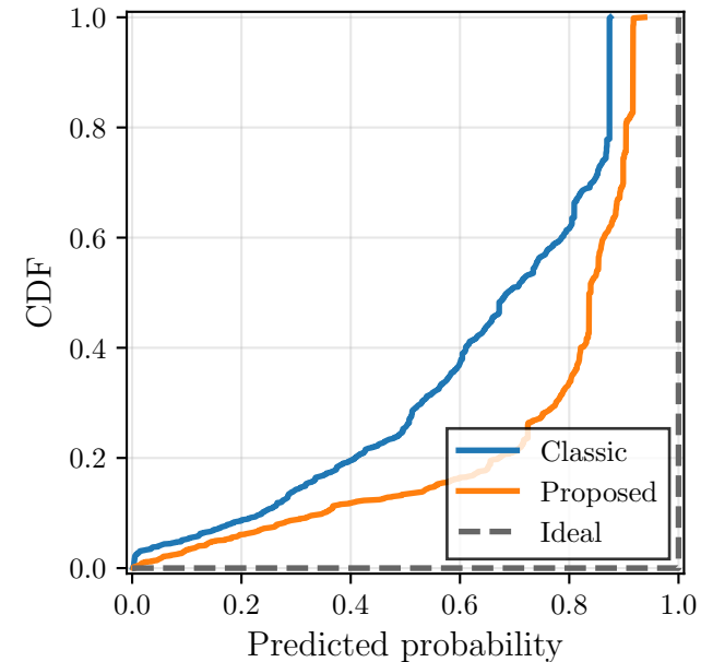
Transaction amount \geq 80
