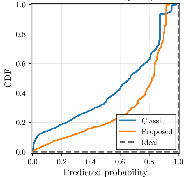
All fraud cases ( y = 1 )
