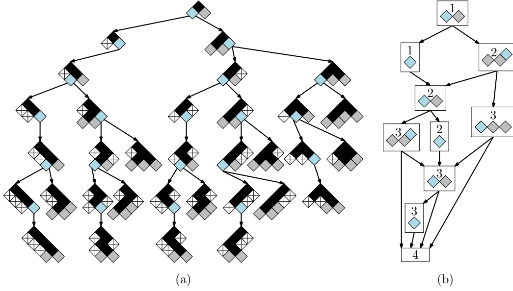
618 Figure 5 (a) an enumeration tree T for directed animals and (b) the associated dynamic- 619 programming DAG G , adapted from Conway [10, Fig. 1 and 2]
