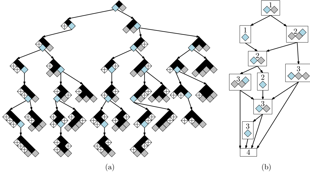
619 Figure 5 (a) an enumeration tree T for directed animals and (b) the associated dynamic- 620 programming DAG G , adapted from Conway [10, Fig. 1 and 2]
