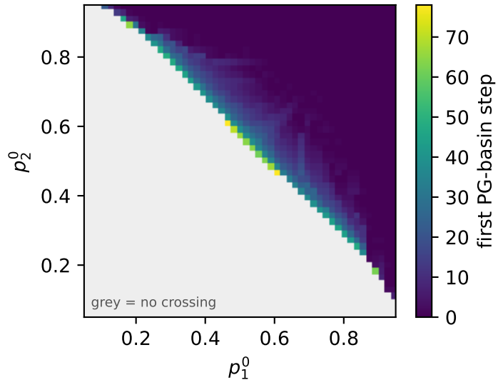
Minimal Meta-MAPG warm-up
