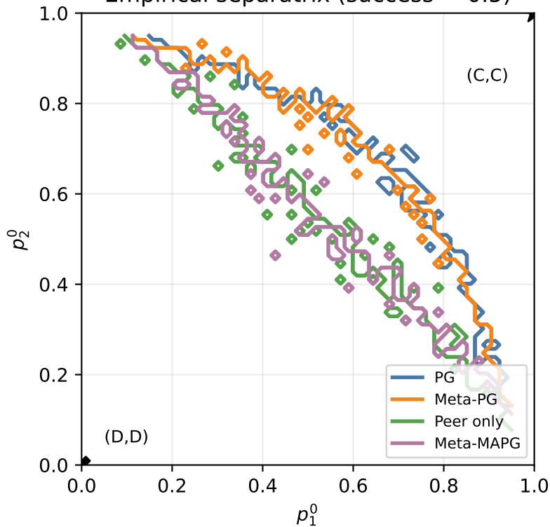
Empirical separatrix (success = 0.5)
