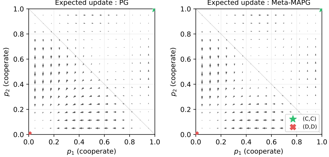
Figure 1: Expected update directions in tabular Stag Hunt. Around the PG separatrix the Meta-MAPG arrows tilt visibly toward the payoff-dominant equilibrium (C, C) , which is the local mechanism behind the basin shifts in Phases B and C.
