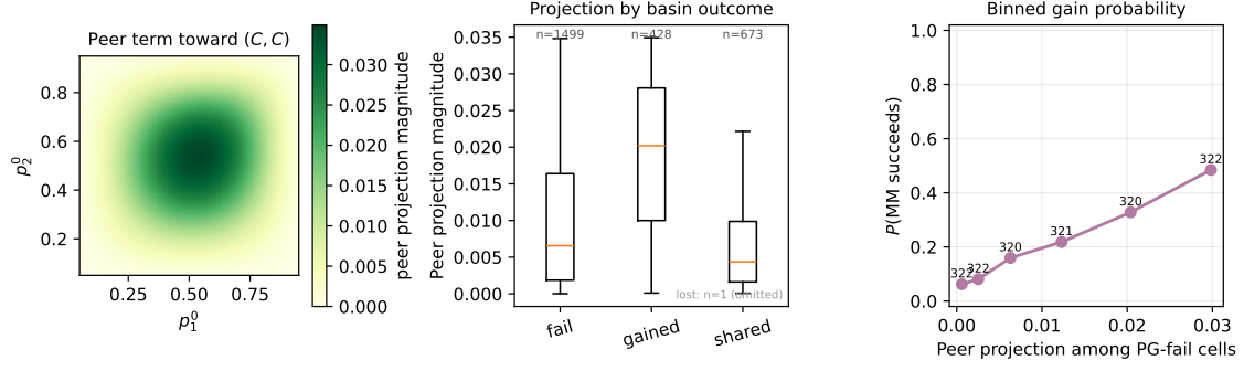
Figure 8: Alignment-to-entry regression. Left: exact peer-correction projection magnitude toward (C, C) (sequential colourmap since all values are non-negative in Stag Hunt). Middle: projection distribution by basin outcome; counts annotated, lost category ( n = 1 ) omitted. Right: binned probability that Meta-MAPG succeeds among cells where PG fails; numbers above dots are bin sizes.
