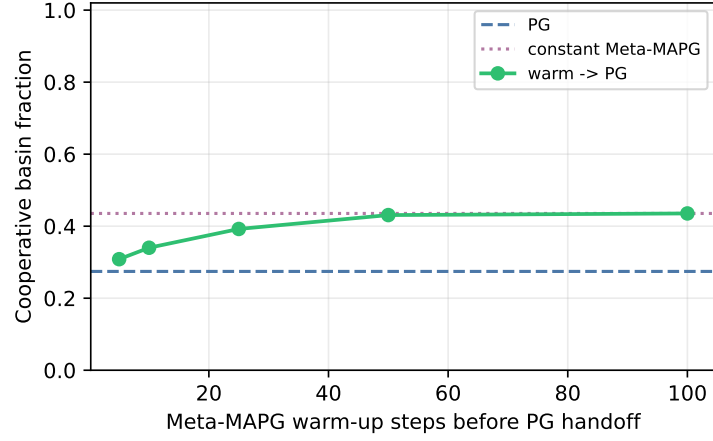
Figure 16: Warm-up handoff curve. Meta-MAPG is used only for the first K steps, followed by pure PG.
