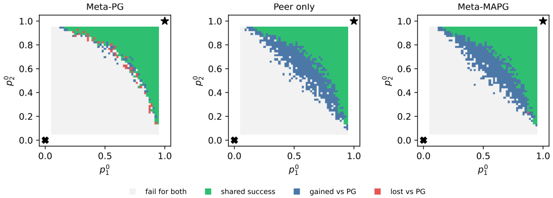
Figure 15: Basin gain/loss masks relative to PG. Peer-only and Meta-MAPG add a large contiguous region below the PG frontier, while Meta-PG adds almost nothing.
