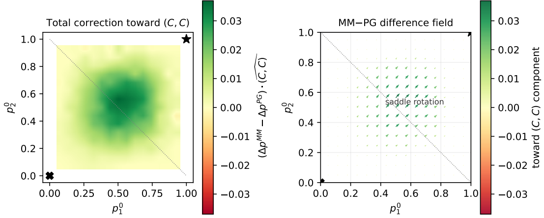
Figure 7: Total Meta-MAPG-minus-PG correction projected toward (C, C) . Left: the scalar projection (\Delta p^{MM} - \Delta p^{PG}) \cdot \hat{d}_{CC} , which includes both own and peer components. Right: the difference quiver coloured by the same projection. Note that this is a directional quantity (not learning-rate-weighted displacement); see Phase R for the isolated peer component.
