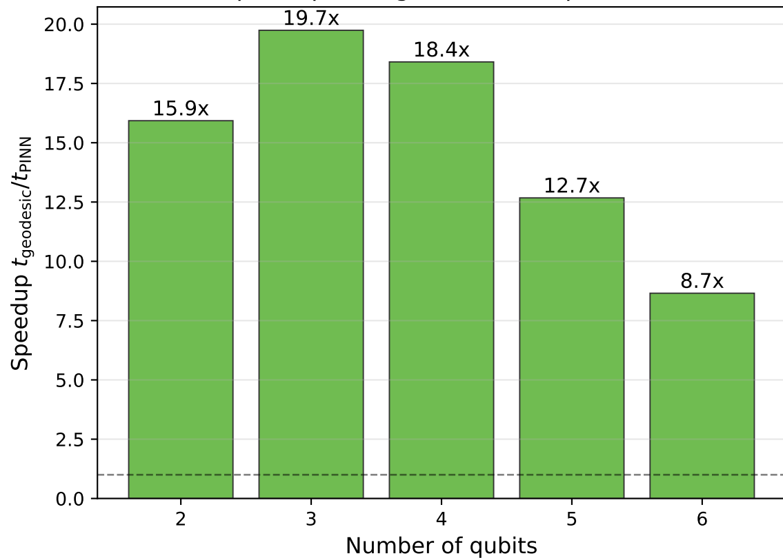
Speedup over geodesic interpolation
