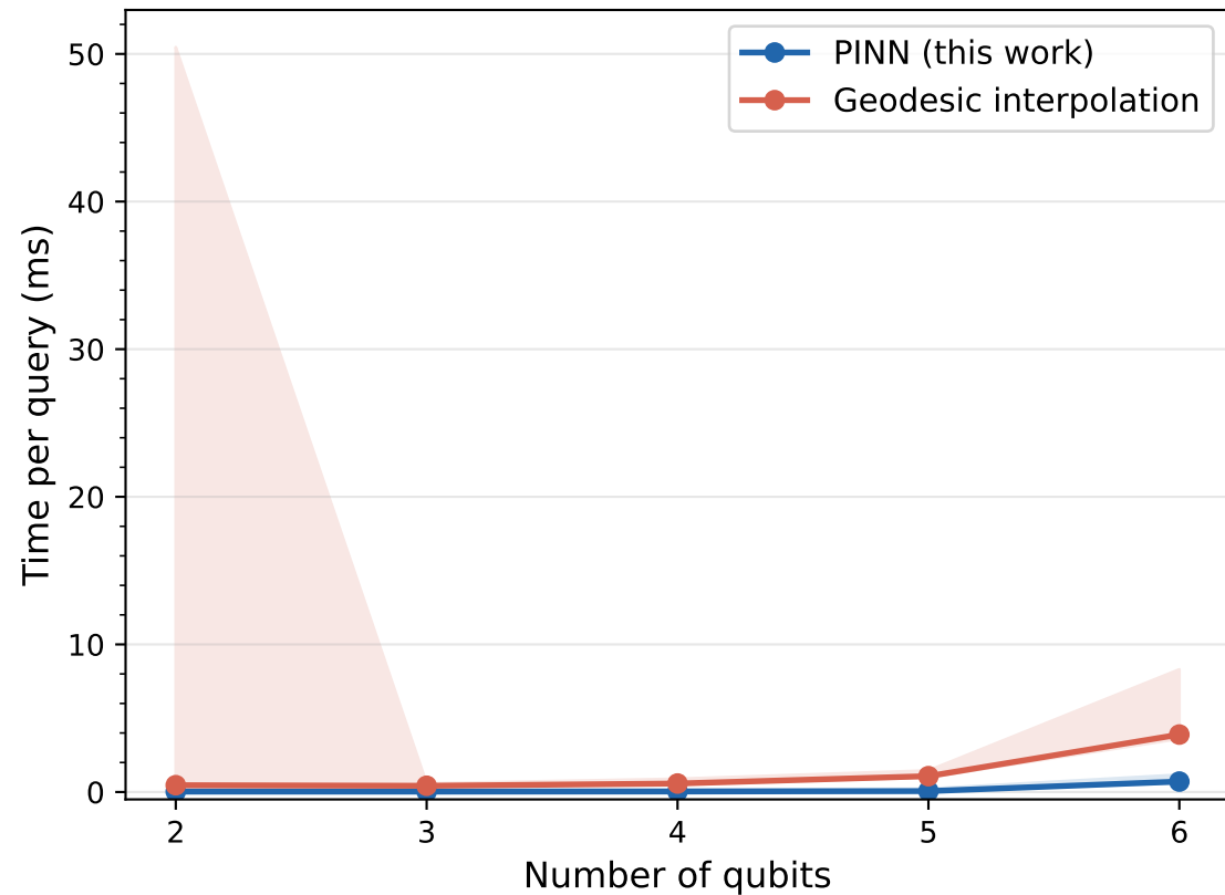
Inference time
