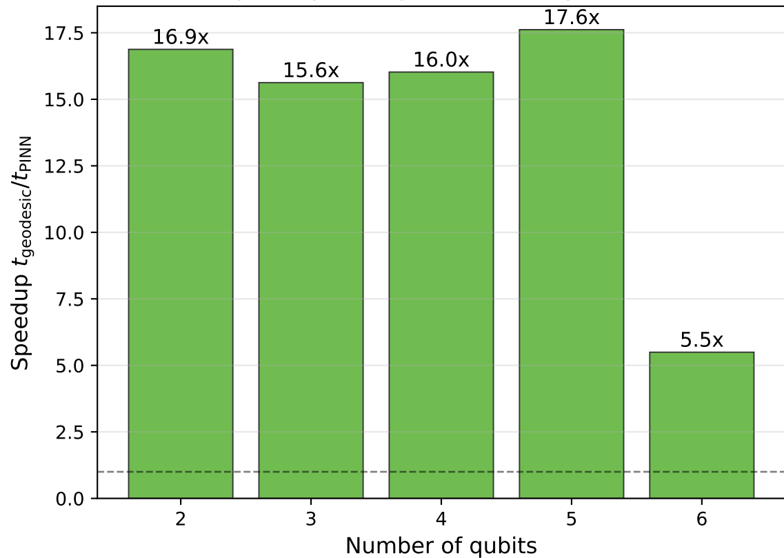
Speedup over geodesic interpolation
