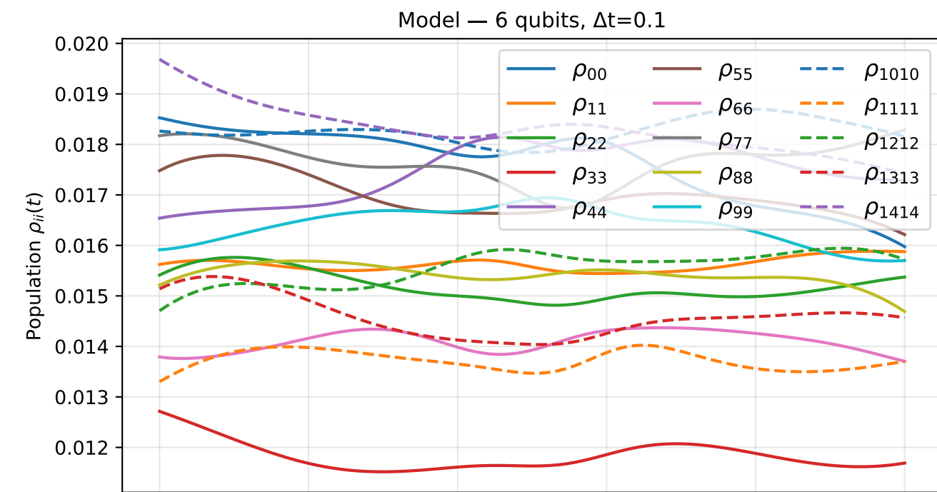
Diagonal elements of \rho(t) — model vs exact (single random initial state)
