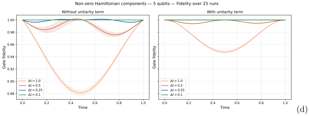
Statistical analysis for the N = 5 qubit case.
