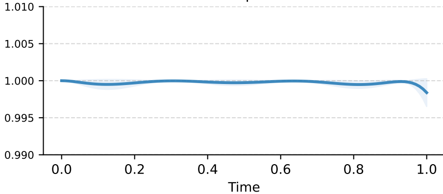
N=7 qubits
