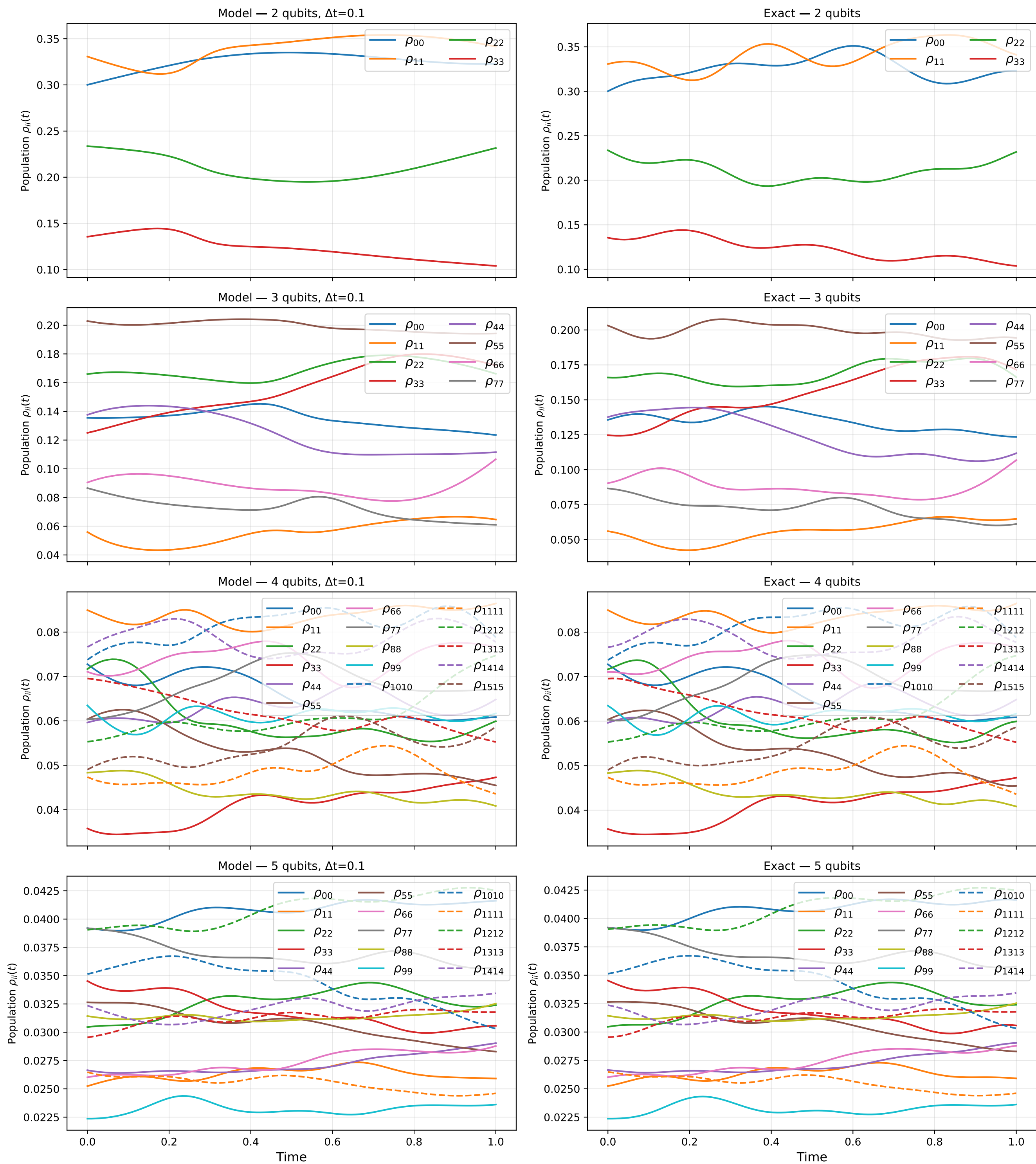
Diagonal elements of \rho(t) — model vs exact (single random initial state)
