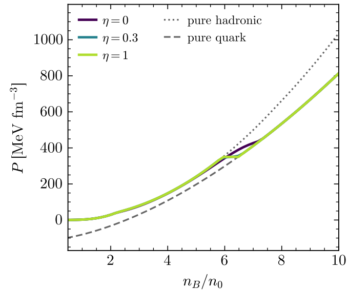
Y_C = 0.1 , T = 0 MeV
