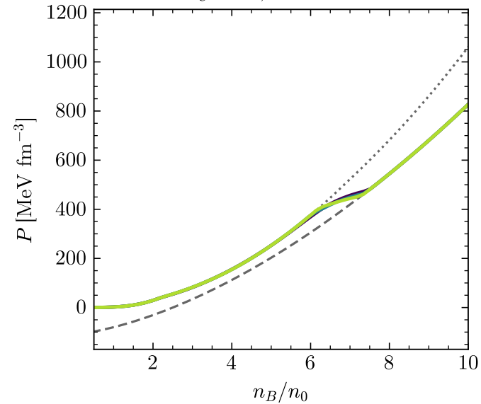
Y_C = 0.1 , T = 0 MeV
