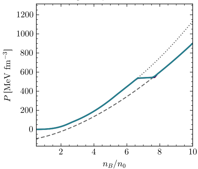
Y_C = 0.4 , T = 0.1 MeV
