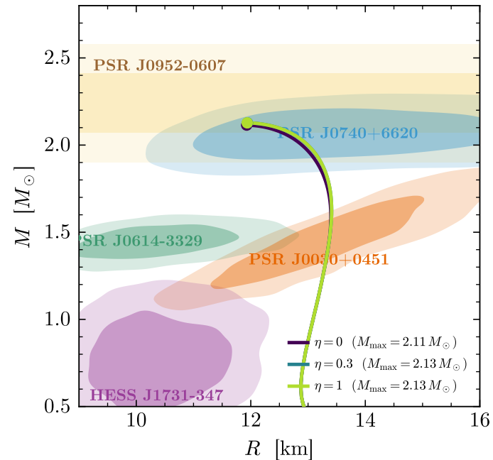
mass-radius
