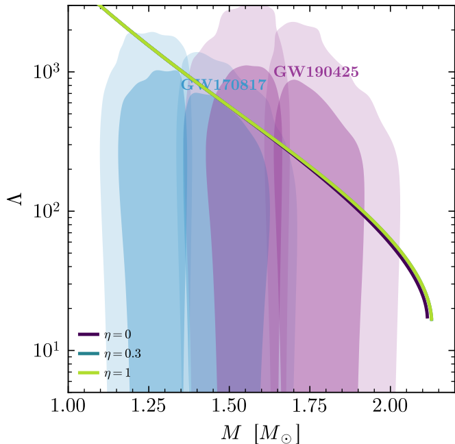
tidal deformability
